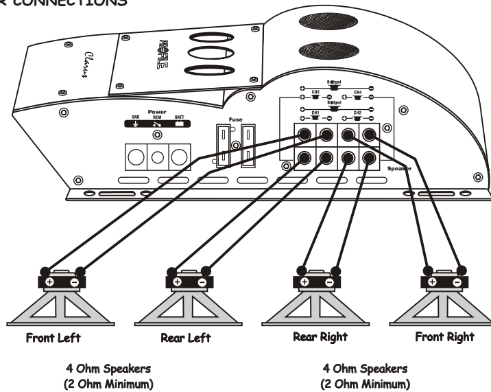
FOUR CHANNEL SPEAKER CONNECTIONS
